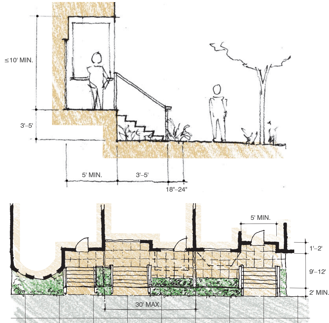
SECTION Dimensions for Ground Floor Exterior Stoop Units
